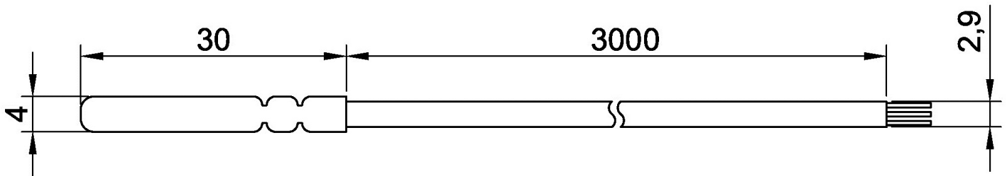
Fig. 2 – The appearance and overall dimensions
