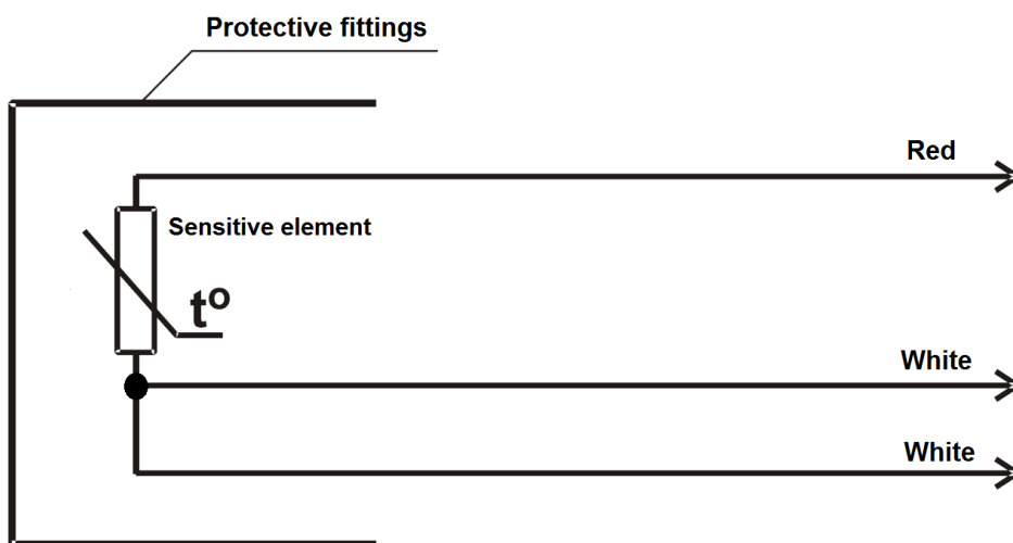
Fig. 1 – Connection diagram
